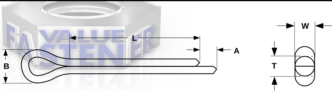
COTTER PINS - EXTENDED PRONG, CHISEL POINT
