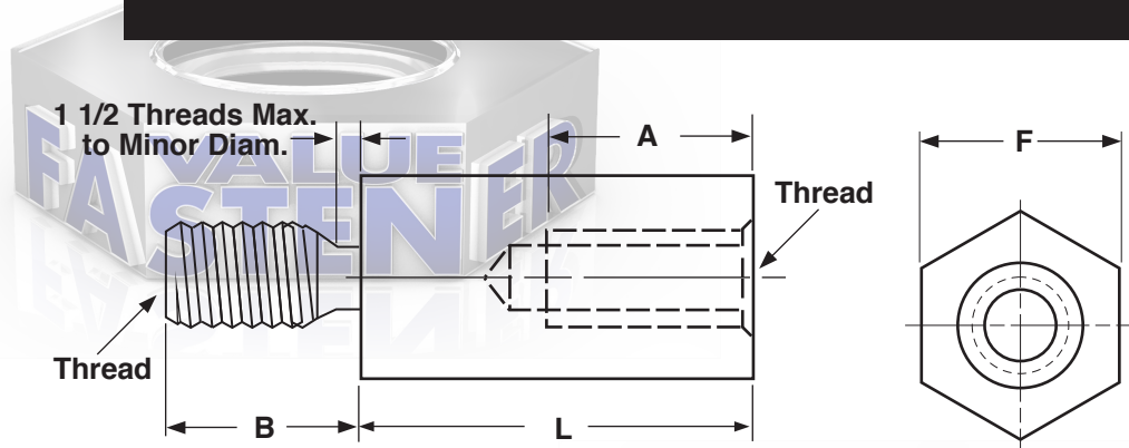
HEXAGON AND ROUND MALE-FEMALE STANDOFFS
