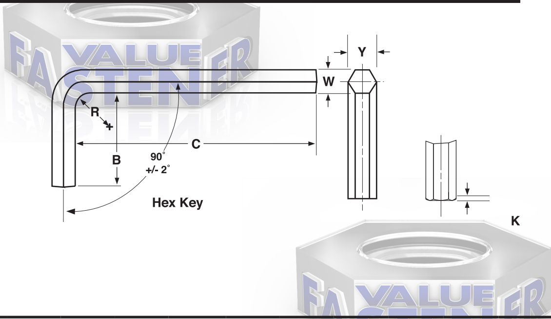
METRIC HEX KEYS, SHORT ARM
